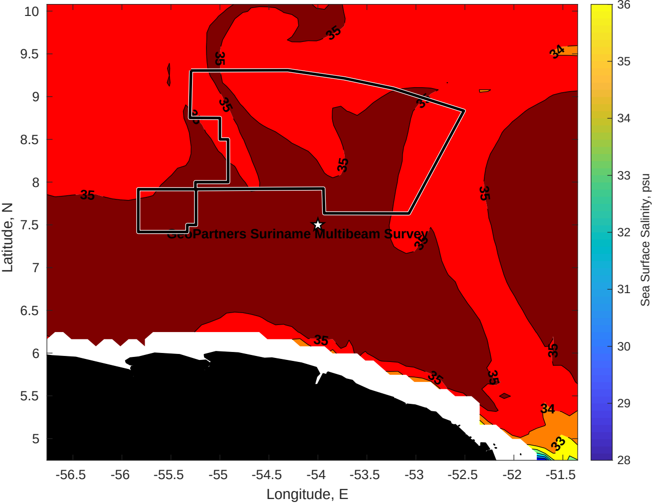
Surface Salinity for GeoPartners Suriname Multibeam Survey at 13-Sep-2024 00:00:00
