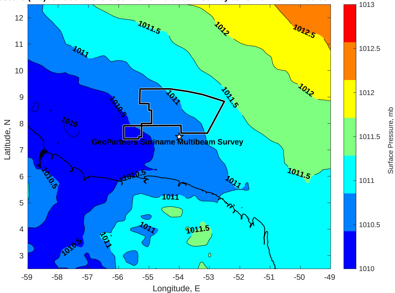
Surface Pressure (mb) for GeoPartners Suriname Multibeam Survey at 15-Nov-2024 12:00:00
