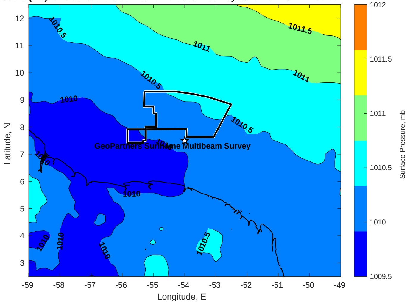
Surface Pressure (mb) for GeoPartners Suriname Multibeam Survey at 16-Nov-2024 12:00:00
