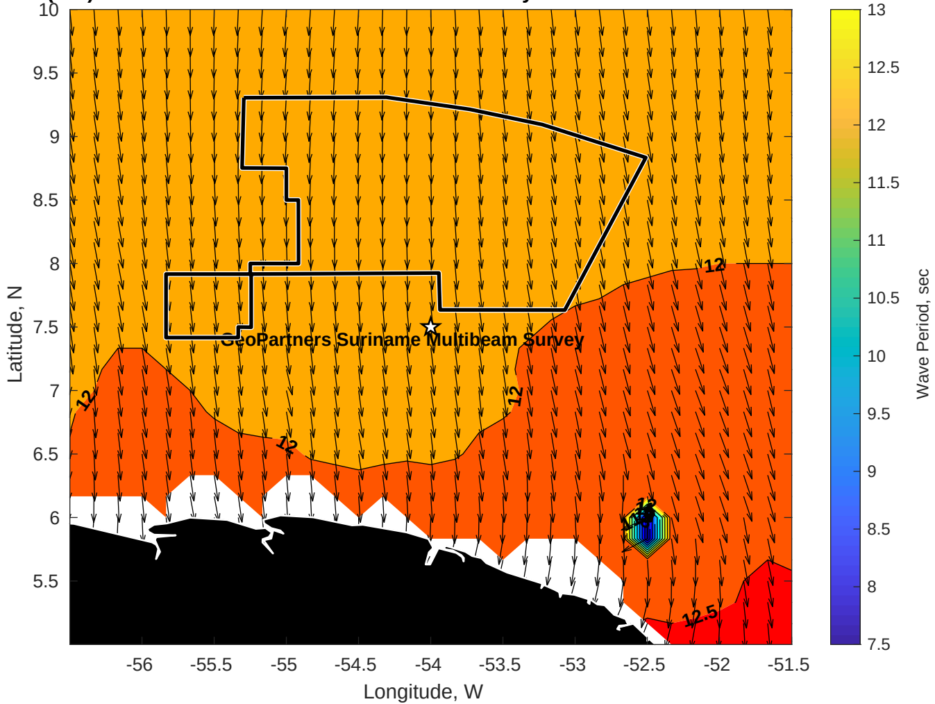
Wave Period (sec) for GeoPartners Suriname Multibeam Survey at 14-Nov-2024 18:00:00
