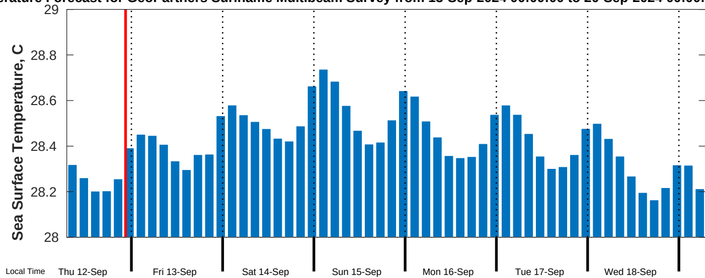
Sea Surface Temperature Forecast for GeoPartners Suriname Multibeam Survey from 13-Sep-2024 00:00:00 to 20-Sep-2024 00:00:00
