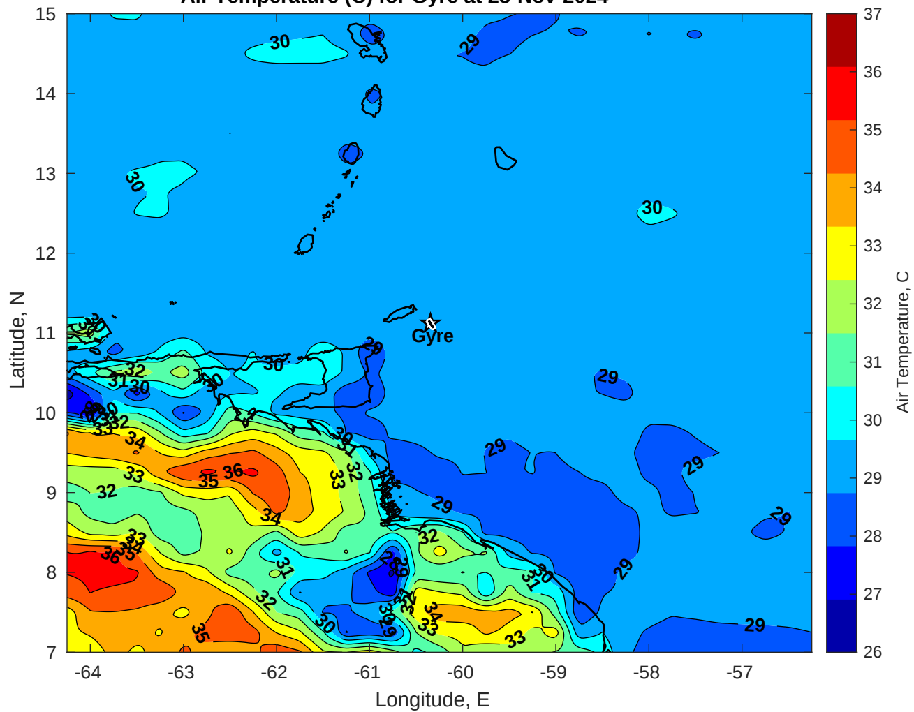
Air Temperature (C) for Gyre at 23-Nov-2024
