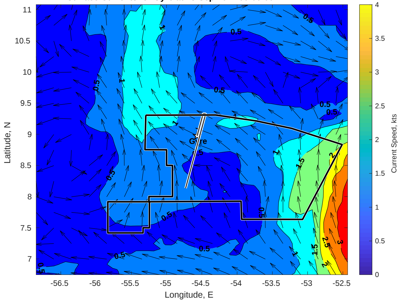
Surface Currents for Gyre at 13-Sep-2024 00:00:00
