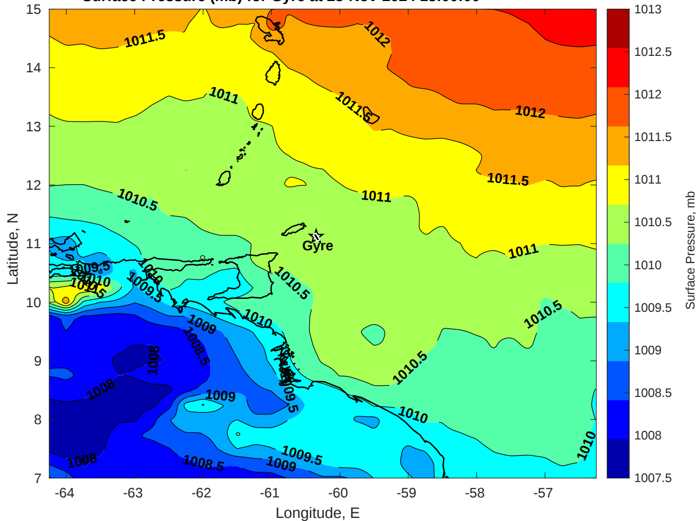
Surface Pressure (mb) for Gyre at 23-Nov-2024 18:00:00
