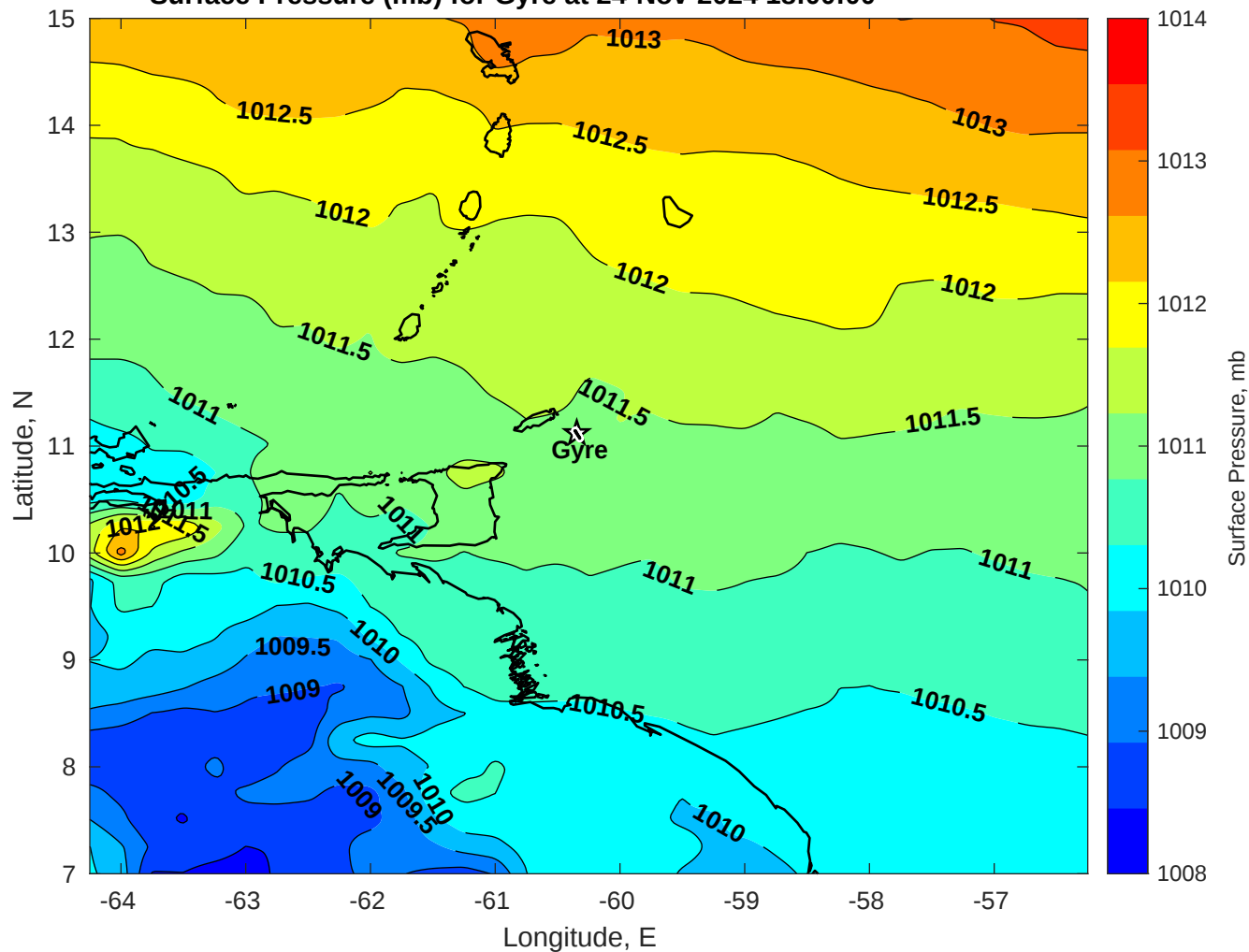
Surface Pressure (mb) for Gyre at 24-Nov-2024 18:00:00
