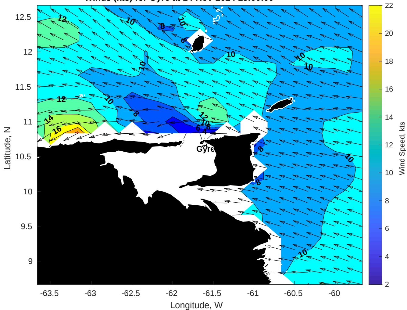
Winds (kts) for Gyre at 14-Nov-2024 18:00:00
