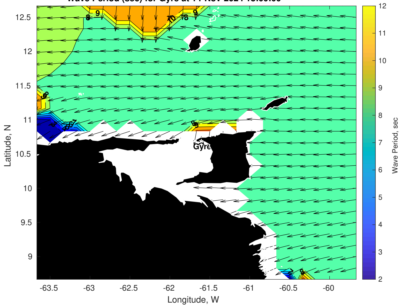
Wave Period (sec) for Gyre at 14-Nov-2024 18:00:00
