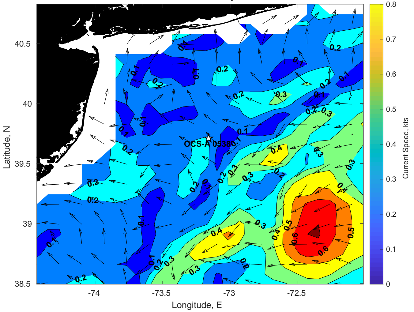
Surface Currents for OCS-A 0538 at 13-Sep-2024 00:00:00
