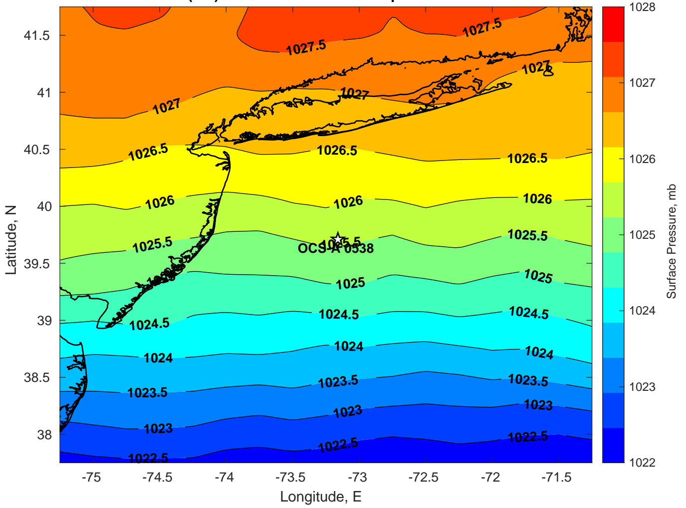
Surface Pressure (mb) for OCS-A 0538 at 16-Sep-2024 06:00:00
