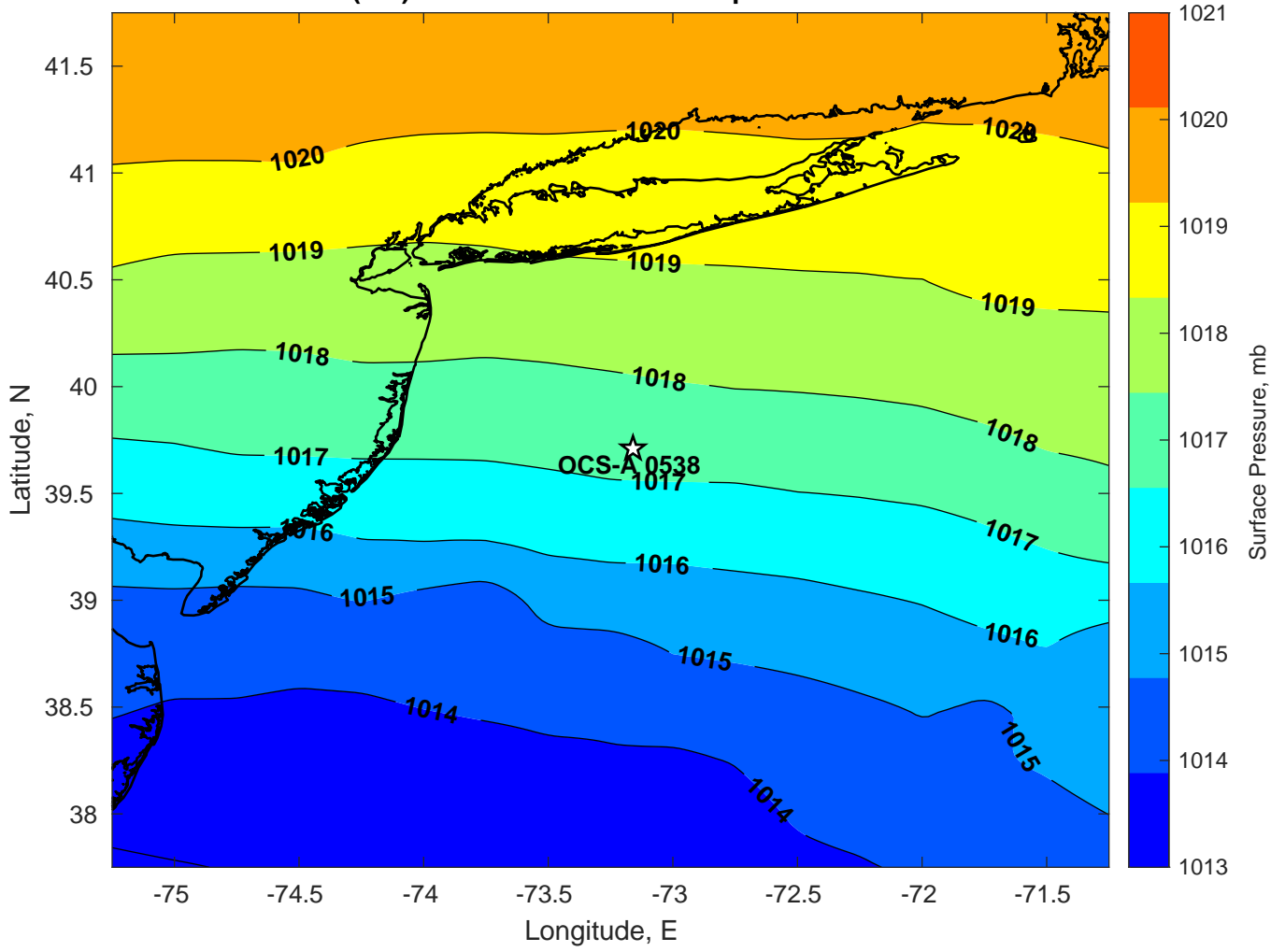
Surface Pressure (mb) for OCS-A 0538 at 18-Sep-2024 06:00:00
