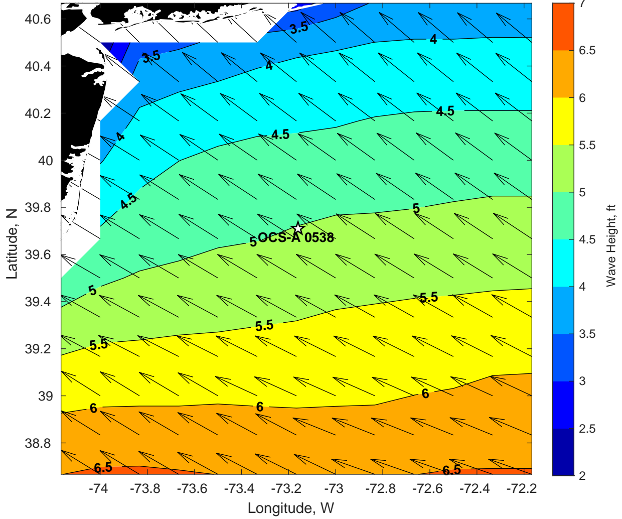
Wave Height (ft) for OCS-A 0538 at 16-Sep-2024 12:00:00
