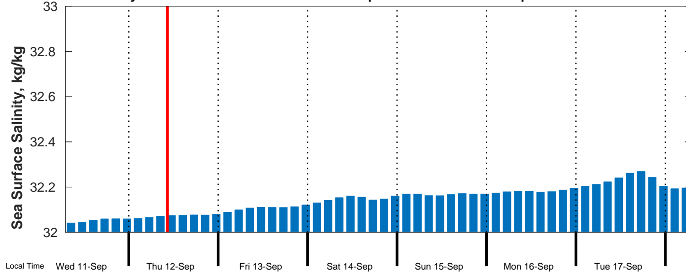
Sea Surface Salinity Forecast for OCS-A 0538 from 12-Sep-2024 00:00:00 to 19-Sep-2024 00:00:00
