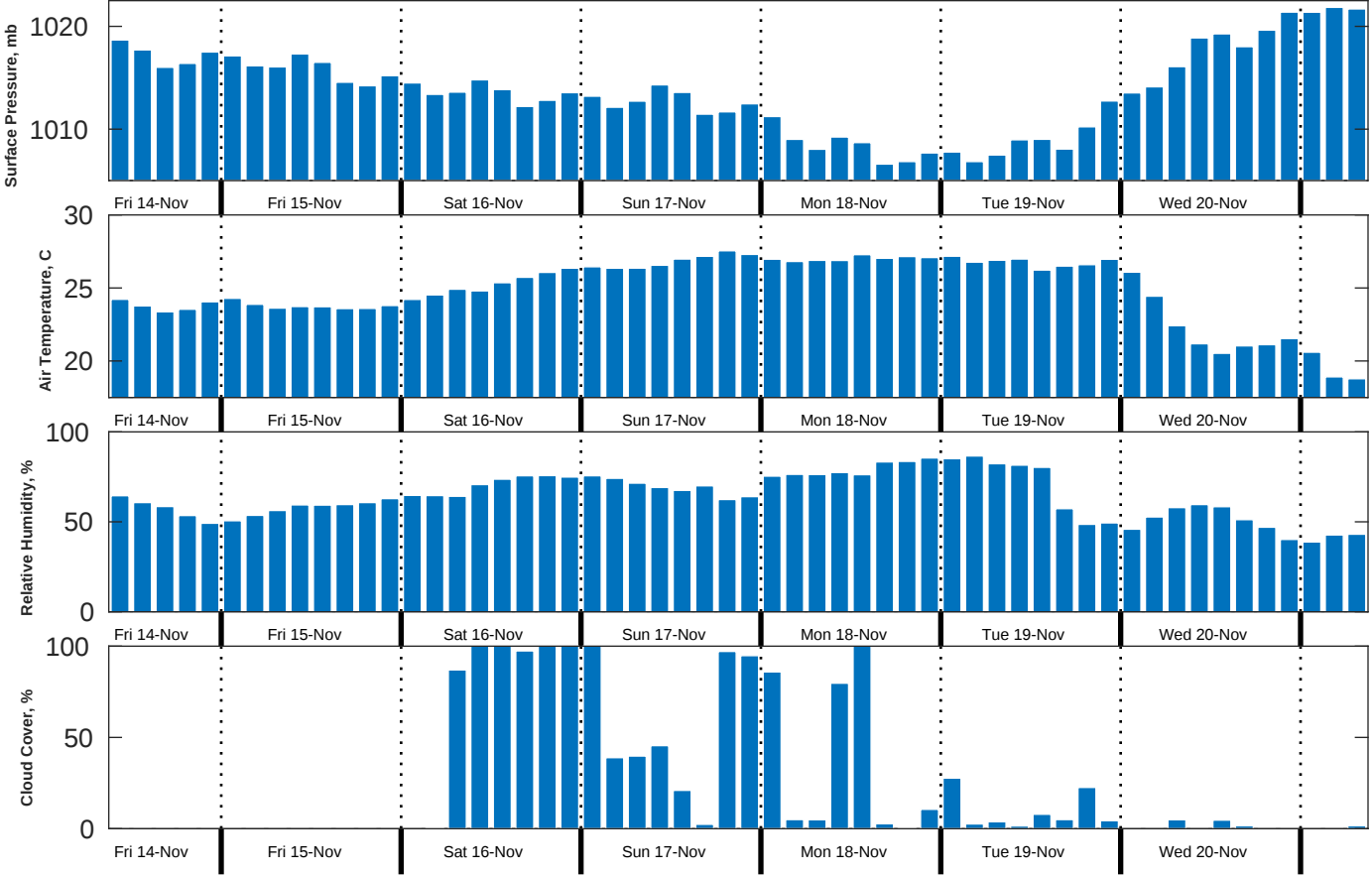
Met Forecast for OXY WOOD Reefing Site (EB125) from 14-Nov-2024 12:00:00 to 21-Nov-2024 12:00:00
