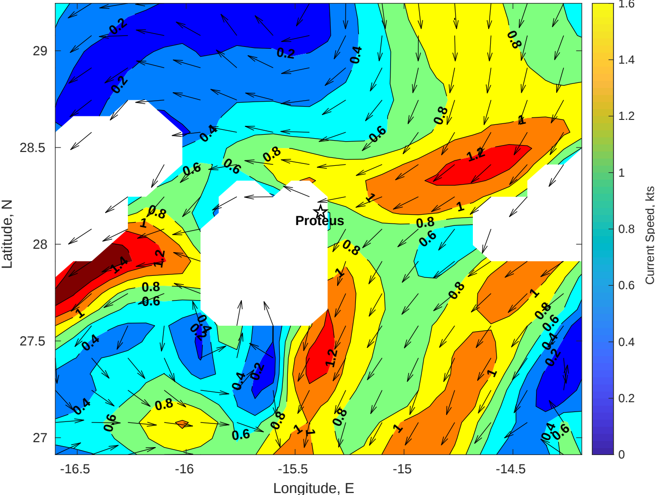
Surface Currents for Proteus at 13-Sep-2024 00:00:00
