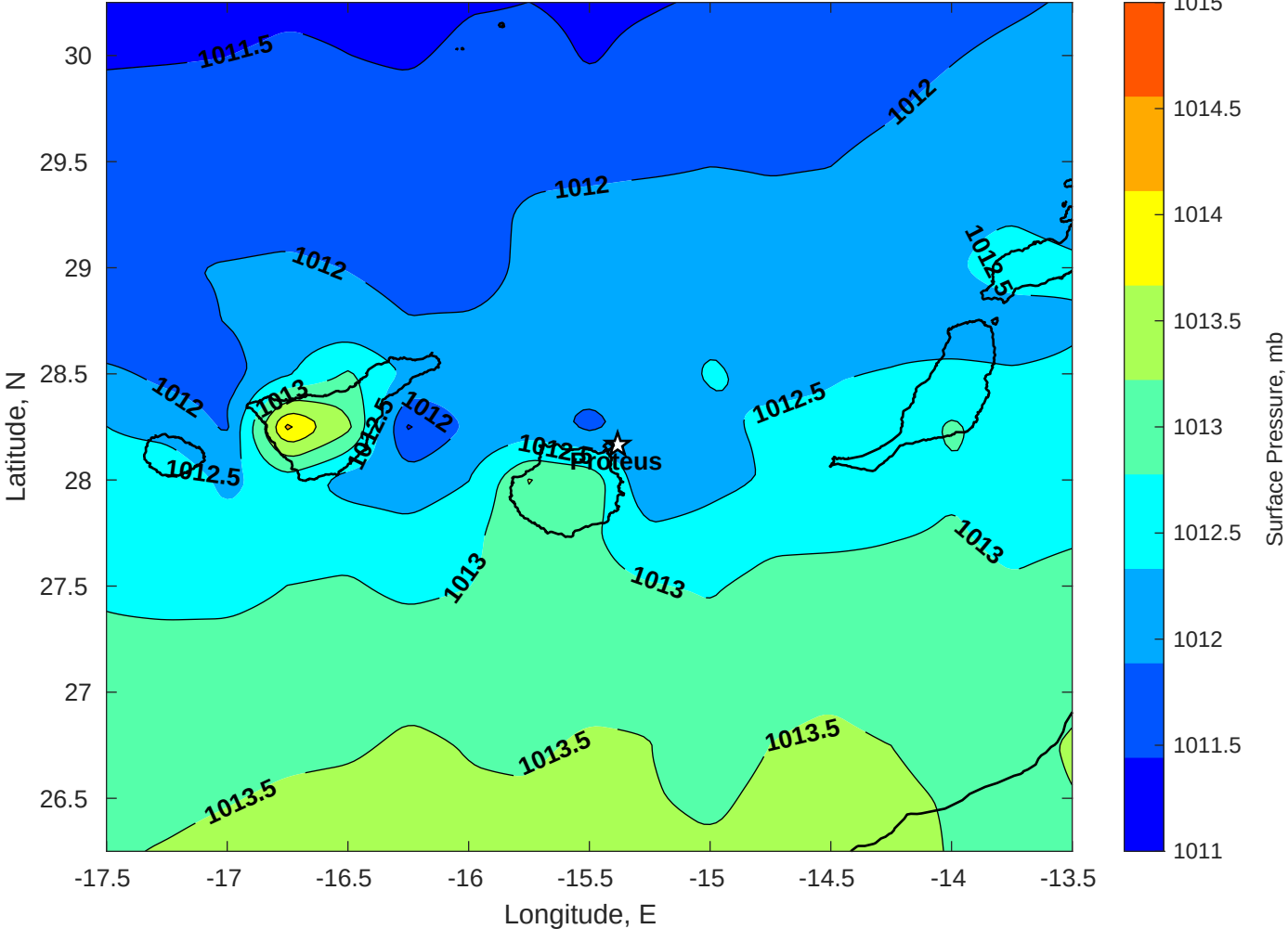
Surface Pressure (mb) for Proteus at 23-Nov-2024 18:00:00
