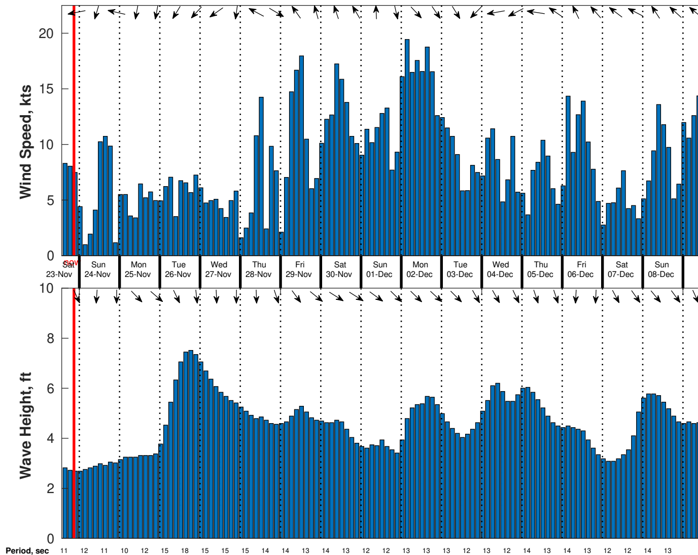
Wind & Wave Forecast for Proteus from 23-Nov-2024 14:00:00 to 09-Dec-2024 14:00:00
