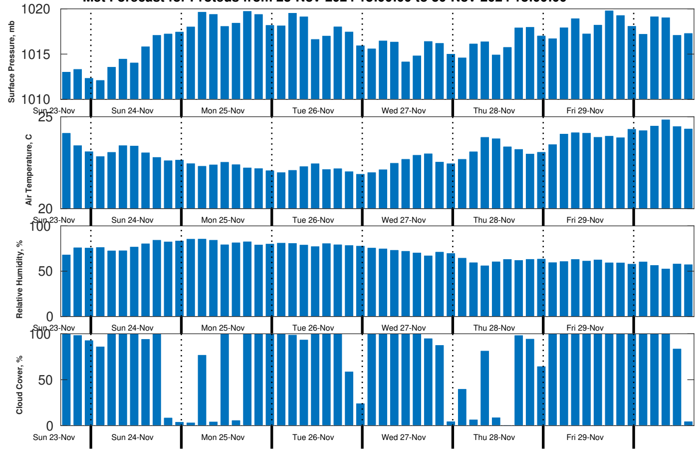
Met Forecast for Proteus from 23-Nov-2024 18:00:00 to 30-Nov-2024 18:00:00
