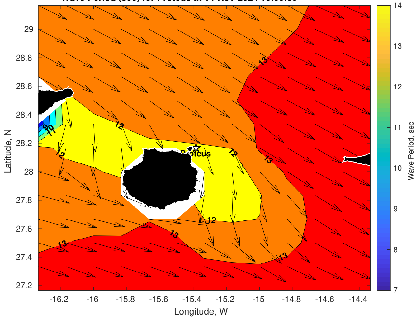
Wave Period (sec) for Proteus at 14-Nov-2024 18:00:00
