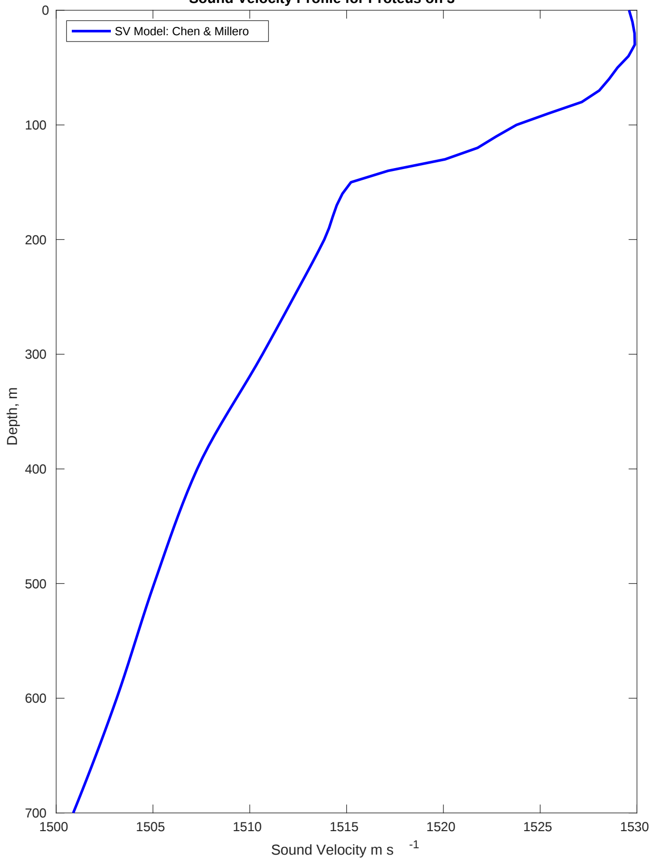
Sound Velocity Profile for Proteus on 3
