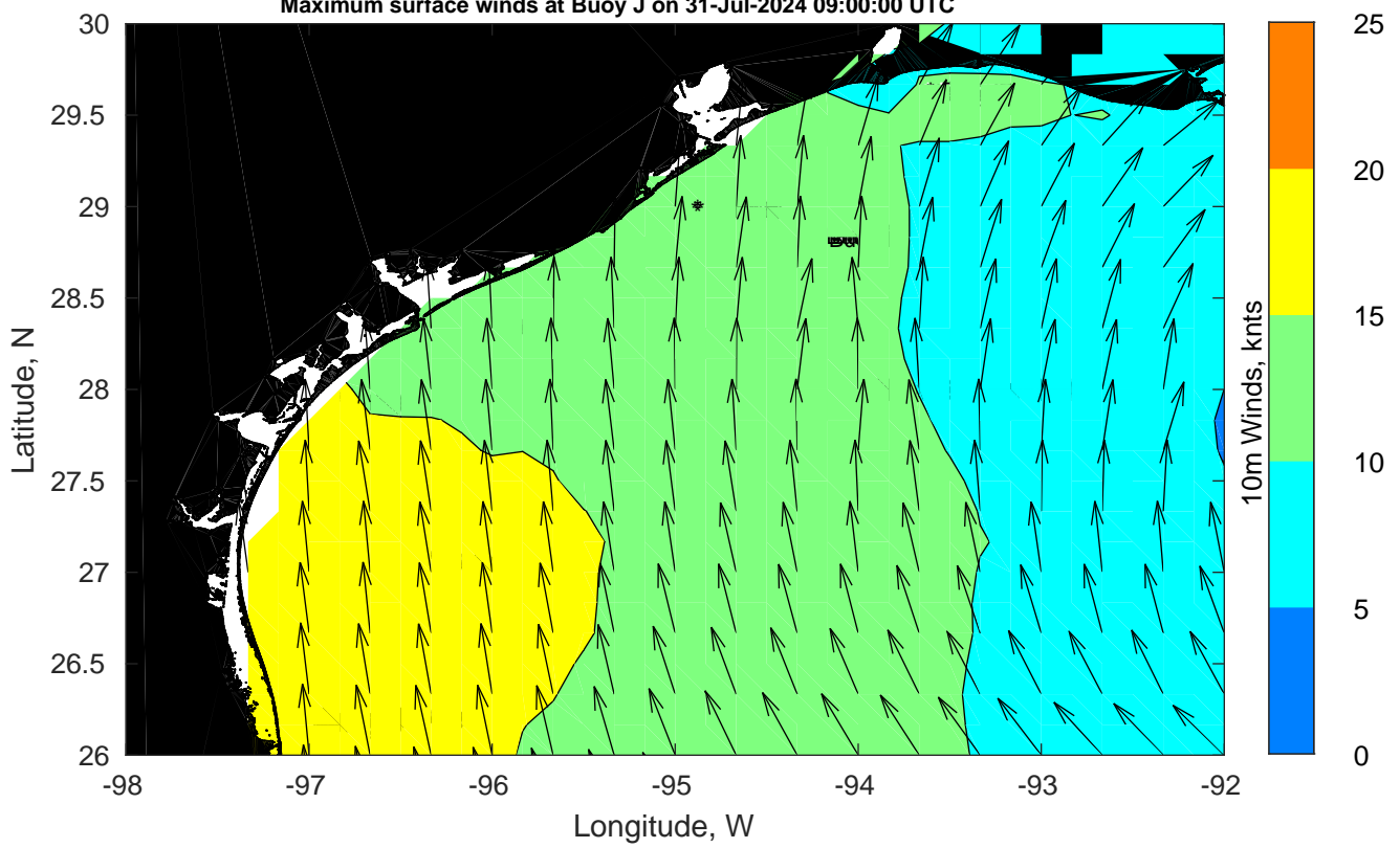
Maximum surface winds at Buoy J on 31-Jul-2024 09:00:00 UTC
